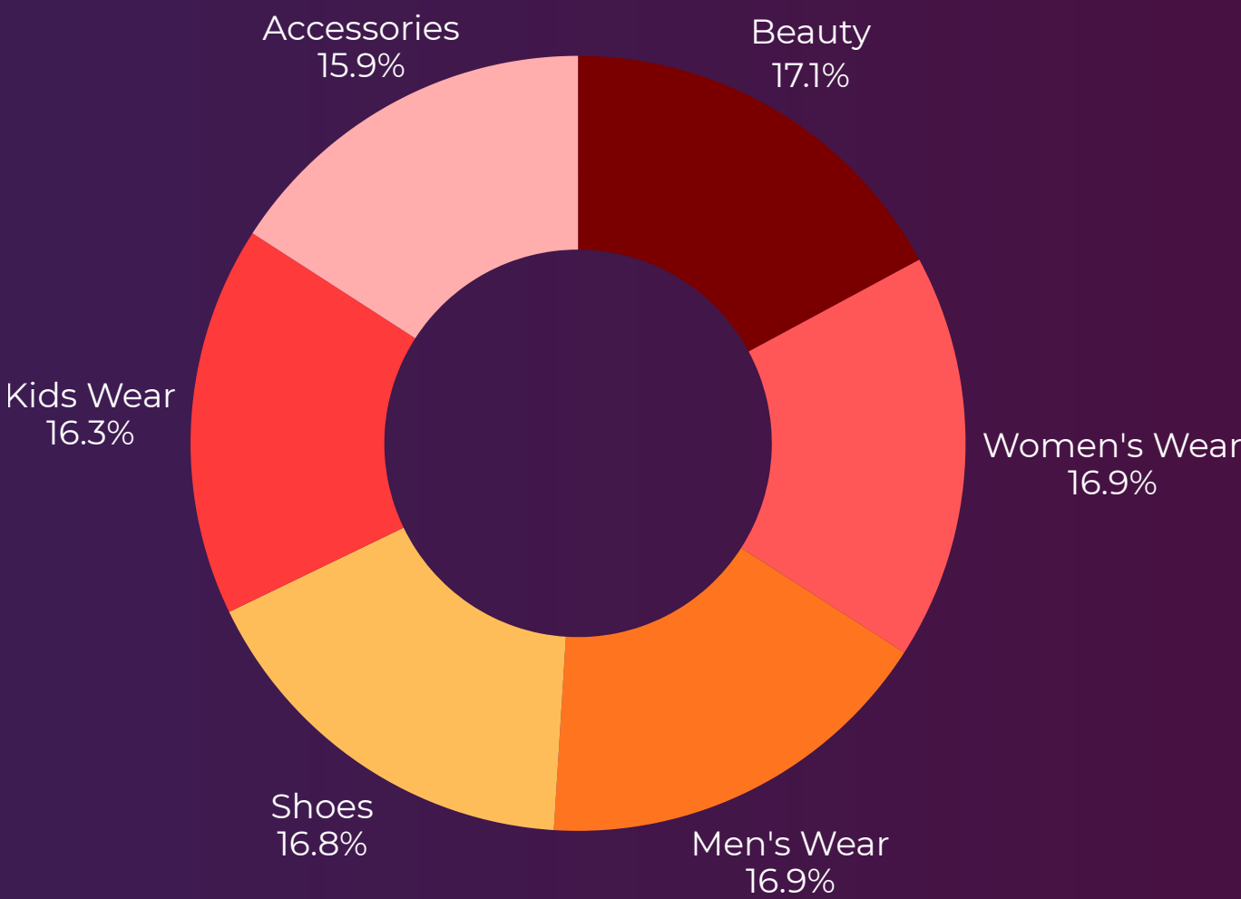
Units Sold
